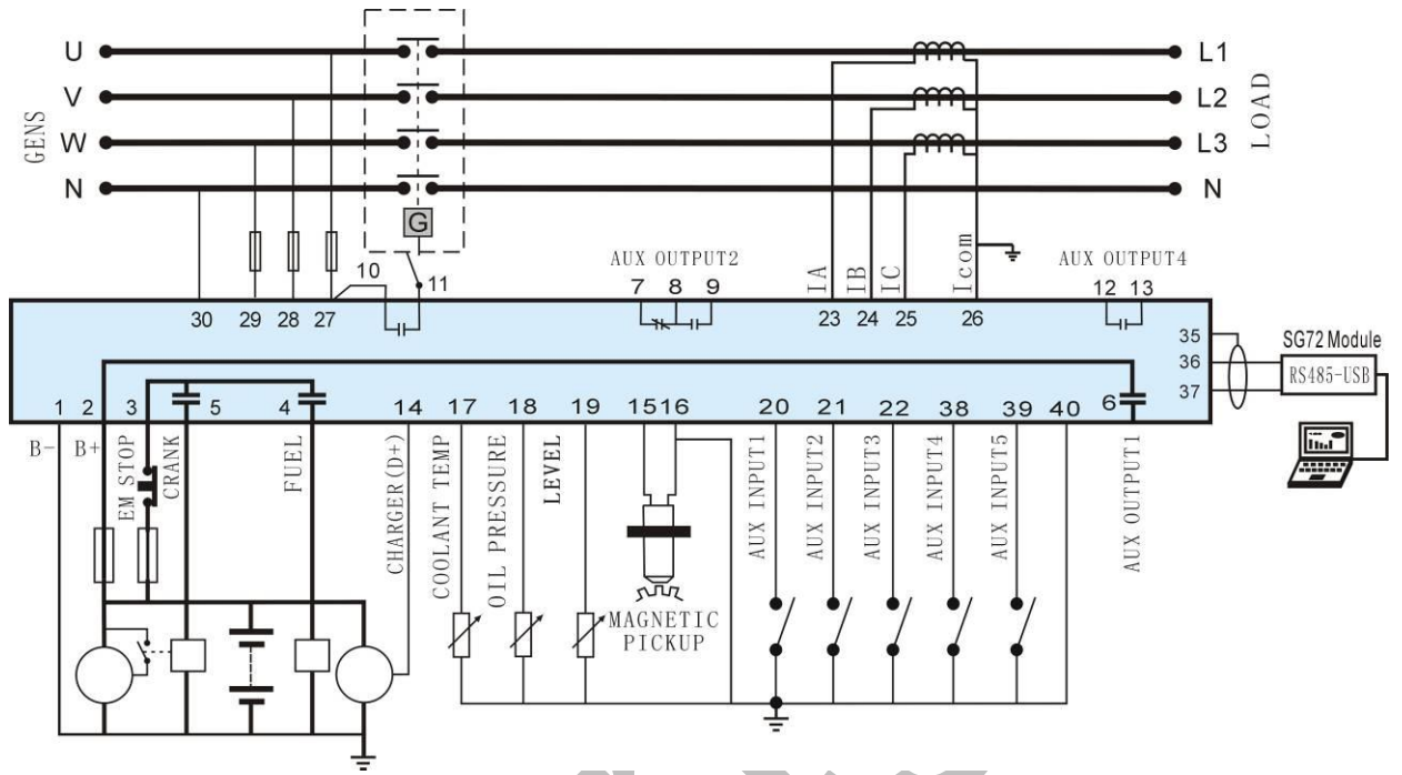
HGM6020KC Typical wiring diagram
