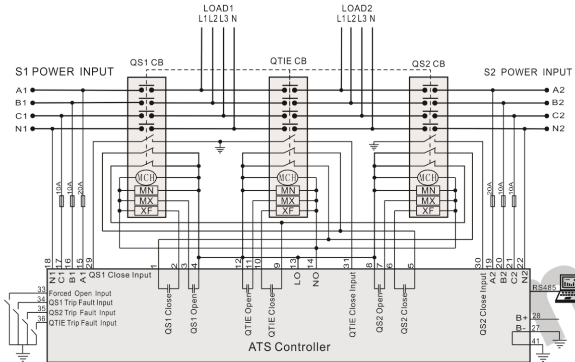
Fig.4 –Breaker Application Diagram 1 (Recommended)
