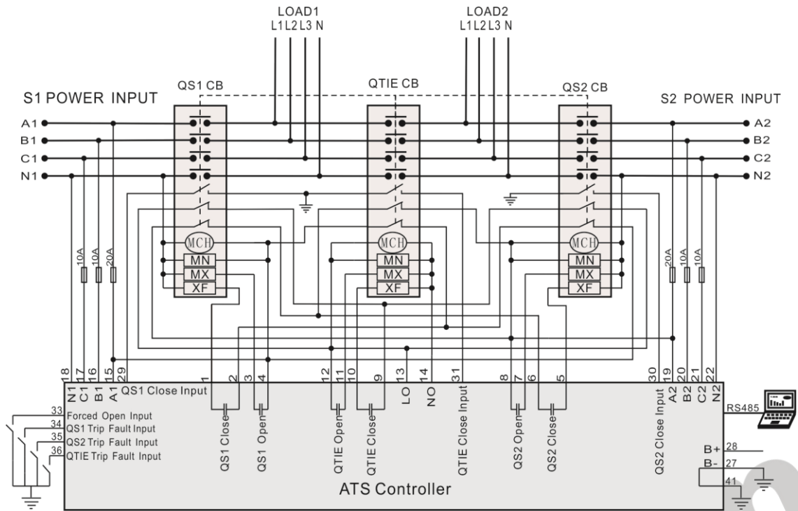
Fig. 5 - Breaker Application Diagram 2
