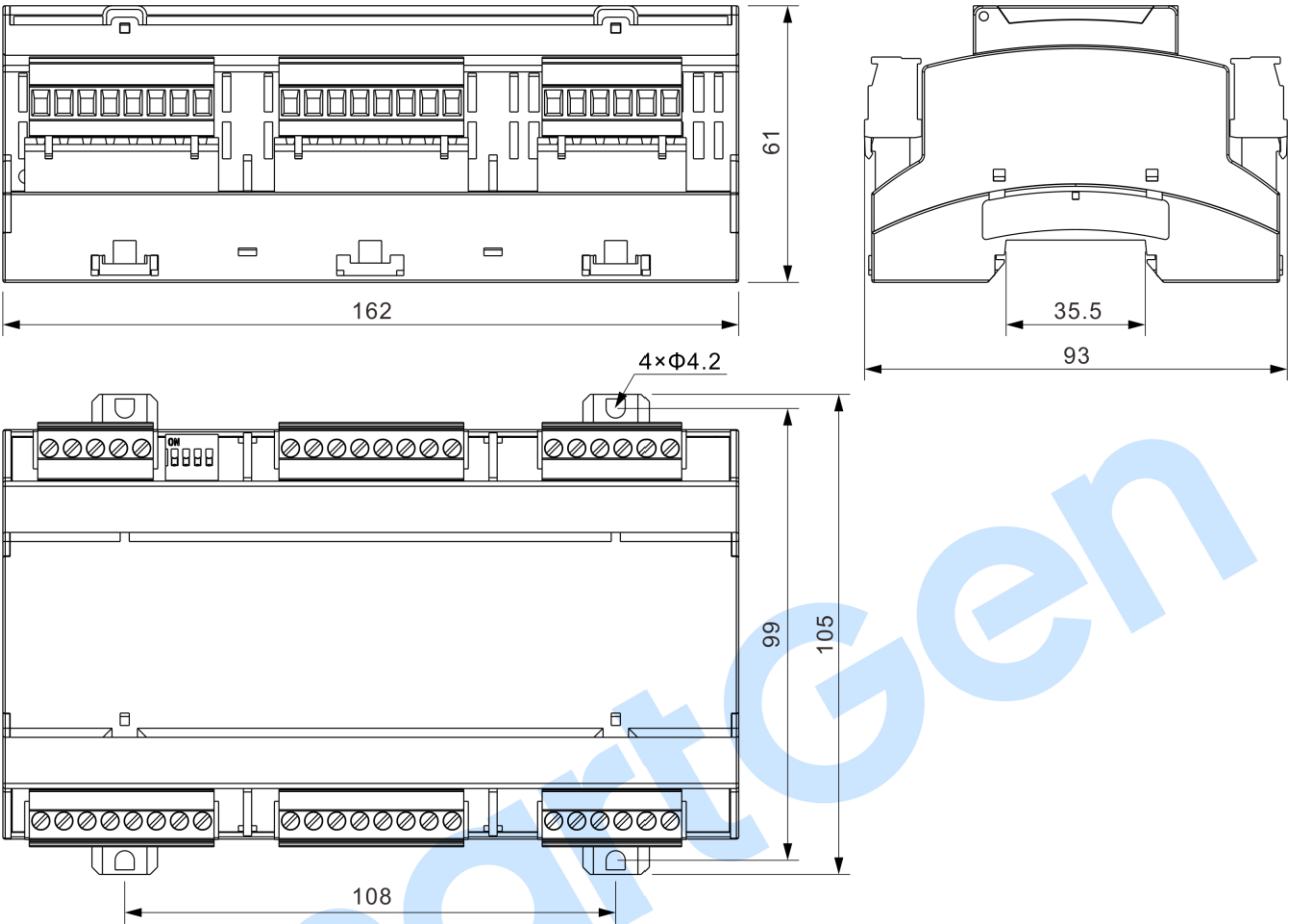
Fig.2 Case Dimensions
